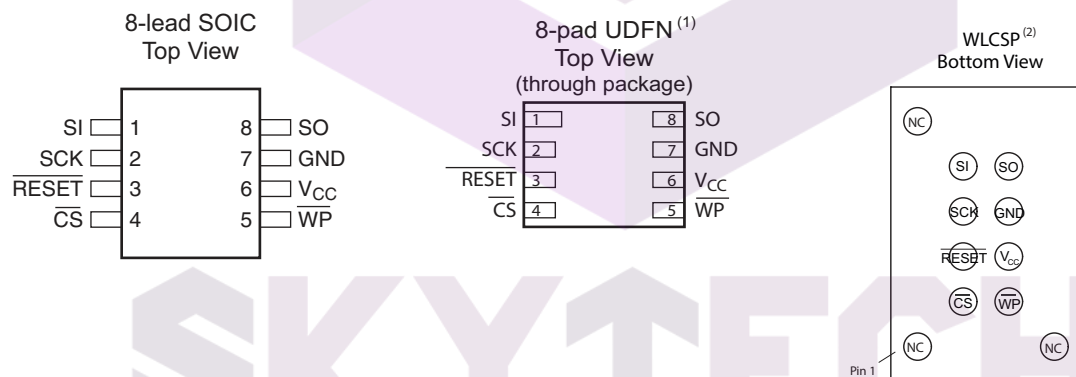
Figure 1-1. Pinouts
