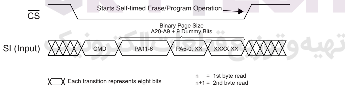
Figure 23-3. Buffer to Main Memory Page Program
